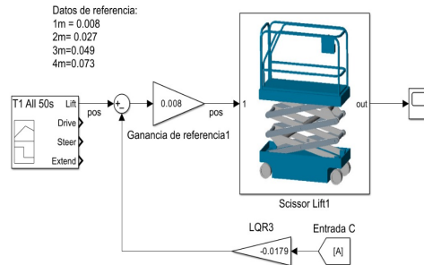
Figure 7: Controlador LQR
