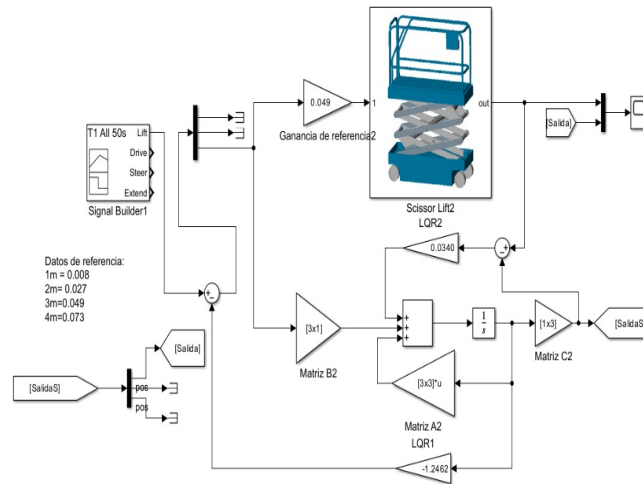
Figure 8: Controlador LQG
